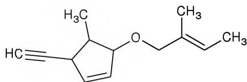
3-ethynyl-4-methyl-5[(2-methylbut-2-en-1-yl)oxy]cyclopentene
