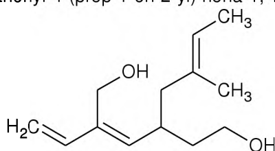
2-ethenyl-4-(2-methylbut-2-en-1-yl) hex-2-ene-1,6-diol
