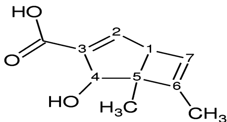
4-hydroxy-5, 6-dimethylbicyclo [3.2.0] hepta-2, 6-diene-3-
