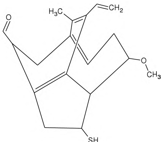
10-ethenyl-5-methoxy-9-methyl-3-sulfanyltricyclo[6.3.2.0 4,11 ]trideca-1(11),7,9-triene-12-carbaldehyde
