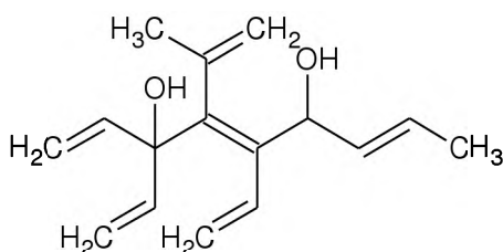
3,5-diethenyl-4-(prop-1-en-2-yl) nona-1,4,7-triene-3,6-diol
