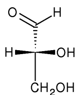
(R)-(+)-Glyceraldehyde
