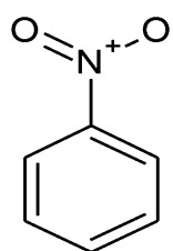
Nitrobenzene
