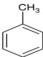
Methylbenzene
